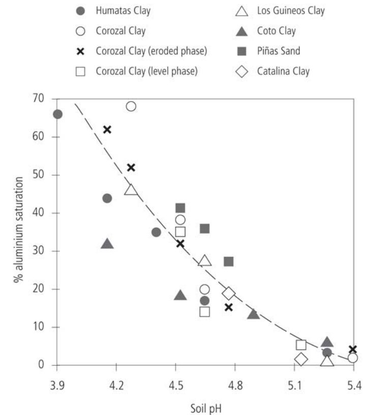
Figure 3. Relationship between soil pH and percent aluminium saturation of the cation exchange complex in eight Puerto Rican soils (Adapted from Bornemiza and Alvarado, 1975)
