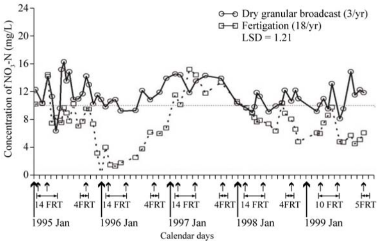
Fig. 6. Concentration of NO 3 -N in the surficial aquifer underneath citrus groves with over-34-year-old “Valencia” orange trees on “Rough lemon” rootstock grown in Astatula fine sand in central Florida. Each data point is the mean of the data from four monitoring well samples (A.K. Alva 2005, unpublished data).
