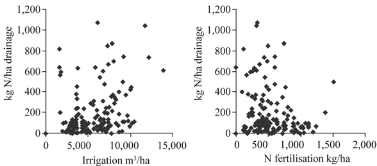
Fig. 2. Relation between the yearly total irrigation (left panel) and the total N fertilisation (right panel) and the total N in the drainage, as monitored in 30 greenhouses during 1996 – 2000 (Voogt, 2003).
