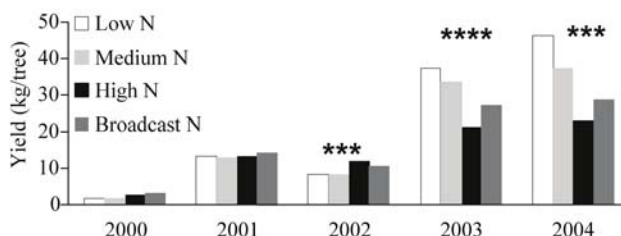
Fig. 5. Yield over five years in Lapins/Gisela 5 sweet cherry trees in response to three levels of fertigated N – (low) 42 mg/L (medium) 84 mg/L, and (high) 168 mg/L – and broadcast N (75 kg/ha).
